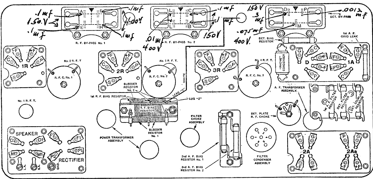
BOTTOM CHART OF LATER-TYPE MODEL 60 AND 60-C.
